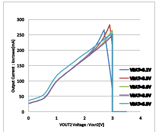
Figure 18. Output Current VS VOUT2 Voltage (VBAT=3.6V,Ta=25°C,VOUT2=3.0V)
