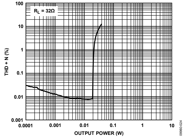
Figure 25. THD + N vs. Output Power into 32Ω, Headphone Amplifier, Stereo Operation
