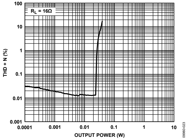
Figure 22. THD + N vs. Output Power into 16Ω, Headphone Amplifier, Stereo Operation
